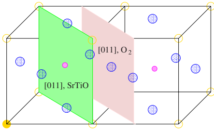
FIG. 2. (Color online) Sketch of the cubic SrTiO 3 perovskite structure showing two (011) cleavage planes that give rise to charged SrTiO and O 2 (011) surfaces.
