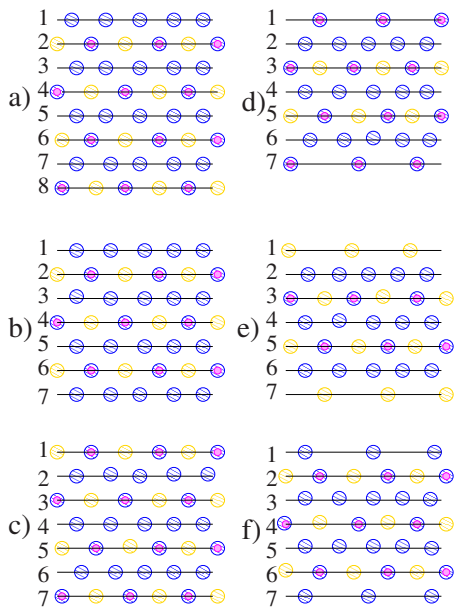
FIG. 3. (Color online) Possible (011) surface slab models considered in the text. [(a)–(c)] Slabs obtained by simple cleavage, yielding mixed, O-terminated, and SrTiO-terminated polar surfaces, respectively. [(d)–(f)] Slabs with nonpolar TiO-terminated, Sr-terminated, and O-terminated surfaces, respectively.
