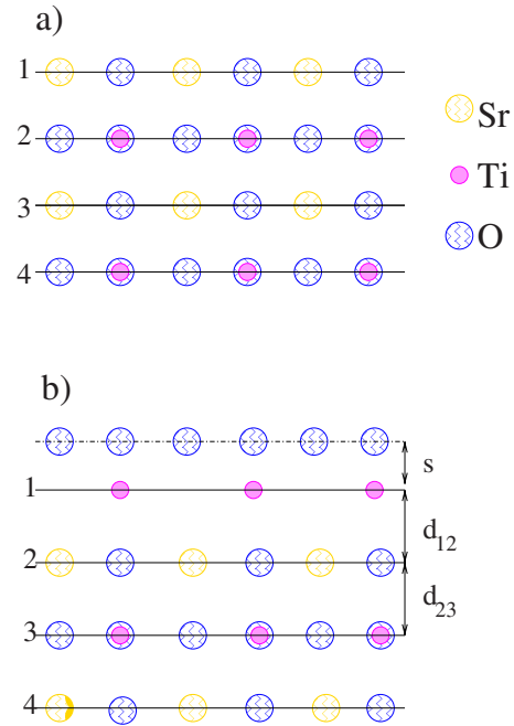
FIG. 1. (Color online) Side view of SrTiO 3 (001) surfaces. (a) SrO-terminated surface. (b) TiO 2 -terminated surface, with definitions of surface rumpling s and the near-surface interplanar separations d_{12} and d_{23} .
