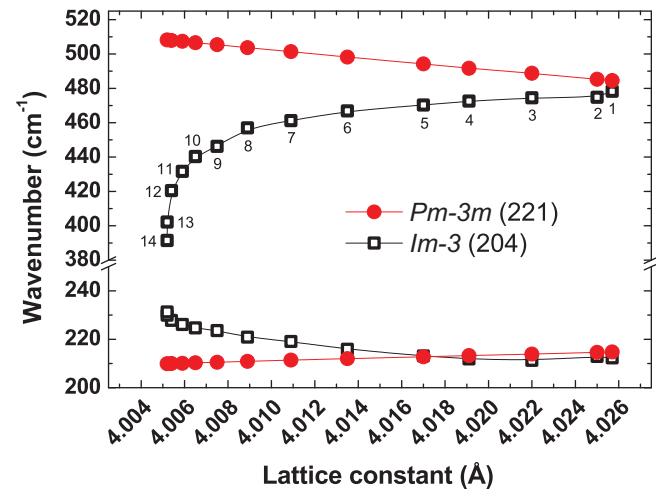
FIG. 8. Variation of the frequencies for IR-active TO phonon modes in \text{ScF}_3 as a function of the lattice parameter in Pm\bar{3}m(221) and Im\bar{3}(204) phases. Points are numbered according to Table I in Supplemental Material [30].
