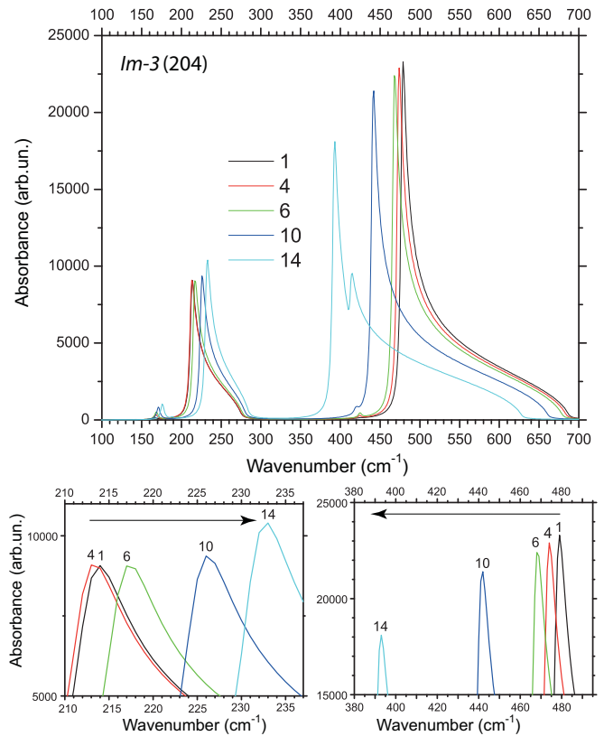
FIG. 7. Calculated infrared absorption spectra of \text{ScF}_3 in Im\bar{3}(204) phase for selected values of contracting lattice parameter a_0 and fluorine atoms displacements. Curves are numbered according to Table I in Supplemental Material [30]. Increasing numbers correspond to higher temperature T and shorter a_0 , as also shown in Fig. 8.
