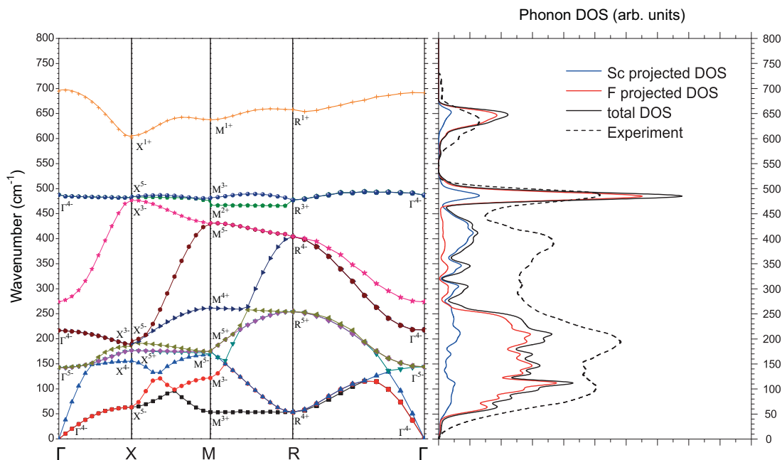
FIG. 5. Calculated phonon dispersions for \text{ScF}_3 in Pm\bar{3}m(221) phase along high-symmetry BZ directions \Gamma -X-M-R- \Gamma (left panel). Total and partial phonon density of states (DOS) obtained from dispersion curves (solid lines) are compared to experimental neutron-weighted phonon DOS at 7 K (black dashed line) adapted from Ref. [4] (right panel).
