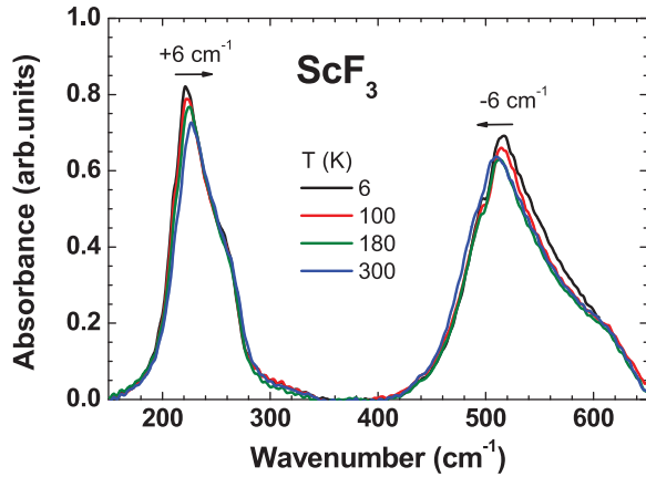
FIG. 2. Experimental infrared absorption spectra of \text{ScF}_3 at selected temperatures. Two bands related to the F–Sc–F bending (at 220 \text{ cm}^{-1} ) and Sc–F stretching (at 520 \text{ cm}^{-1} ) modes are visible. A shift of the band maxima by about 6 \text{ cm}^{-1} in the opposite directions occurs on increasing temperature.
