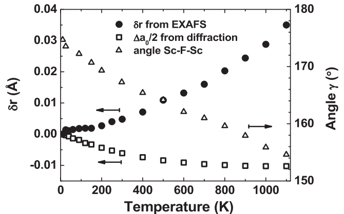
FIG. 4. Temperature dependence of the first coordination shell parameters: \delta r (filled circles) is the bond length Sc-F measured by EXAFS; \Delta a_0/2 (squares) corresponds to half of the lattice parameter obtained by diffraction in Ref. [6]; \gamma (triangles) is the calculated average angle Sc-F-Sc (see Fig. 1).
