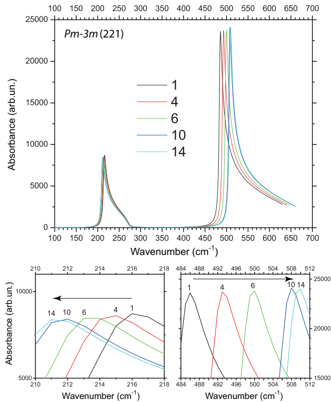
FIG. 6. Calculated infrared absorption spectra of \text{ScF}_3 in Pm\bar{3}m(221) phase for selected values of contracting lattice parameter a_0 . Curves are numbered according to Table I in Supplemental Material [30]. Increasing numbers correspond to higher temperature T and shorter a_0 , as also shown in Fig. 8.
