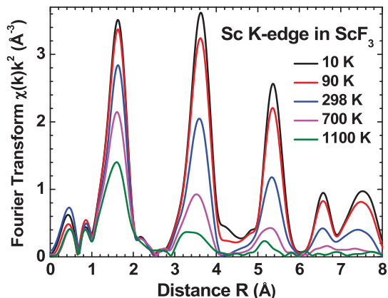
FIG. 3. Fourier transforms of the experimental Sc K-edge EXAFS \chi(k)k^2 for polycrystalline \text{ScF}_3 at selected temperatures from 10 to 1100 K.
