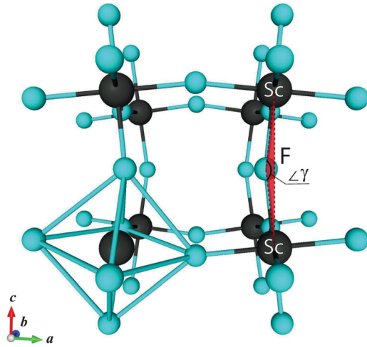
FIG. 1. Schematic view of \text{ScF}_3 structure with librated \text{ScF}_6 octahedra. The tilt angle \text{Sc-F-Sc} is defined as \gamma . (The small balls are fluorine atoms, the large balls are scandium atoms.)
