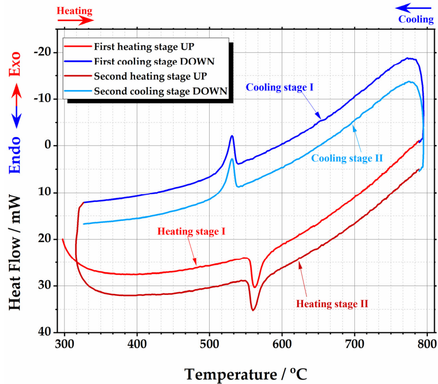
Figure A7. DSC curve of the phase transition cycles for \text{La}_{1.9975}\text{Ti}_{0.0025}\text{Mo}_2\text{O}_{9.00125} ceramic heat-treated at 1000 °C.
