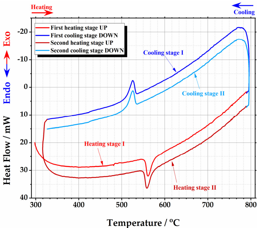
Figure A1. DSC curve of the phase transition cycles for \text{La}_{1.99975}\text{Ti}_{0.00025}\text{Mo}_2\text{O}_{9.000125} ceramic heat-treated at 1000 °C.
