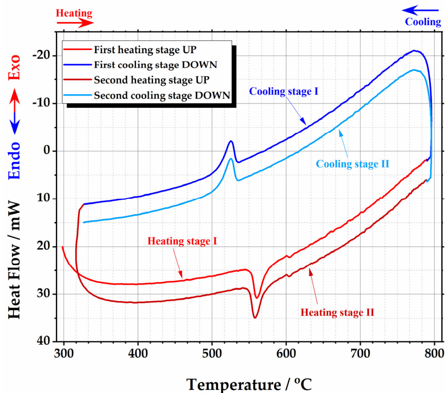
Figure A2. DSC curve of the phase transition cycles for \text{La}_{1.9995}\text{Ti}_{0.0005}\text{Mo}_2\text{O}_{9.00025} ceramic heat-treated at 1000 °C.
