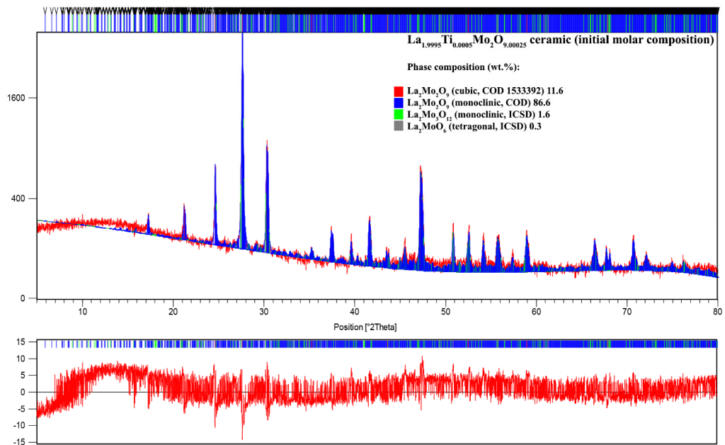
Figure A10. XRD pattern processed by Rietveld refinement for the \text{La}_{1.9995}\text{Ti}_{0.0005}\text{Mo}_2\text{O}_9 ceramic composition.
