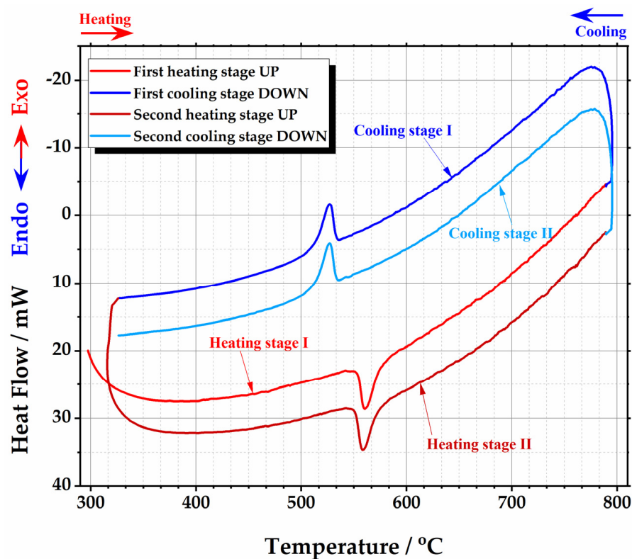
Figure A4. DSC curve of the phase transition cycles for \text{La}_{1.999}\text{Ti}_{0.001}\text{Mo}_2\text{O}_{9.0005} ceramic heat-treated at 1000 °C.
