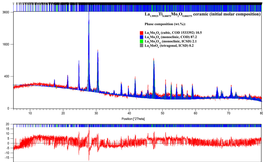
Figure A11. XRD pattern processed by Rietveld refinement for the \text{La}_{1.99925}\text{Ti}_{0.00075}\text{Mo}_2\text{O}_9 ceramic composition.
