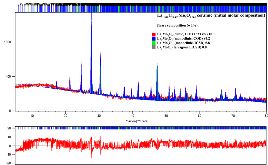
Figure A14. XRD pattern processed by Rietveld refinement for the La 1.998 Ti 0.002 Mo 2 O 9.001 ceramic composition.
