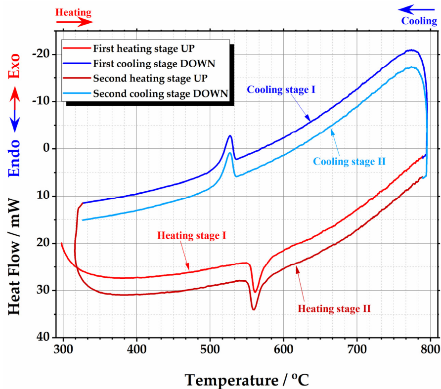
Figure A6. DSC curve of the phase transition cycles for \text{La}_{1.998}\text{Ti}_{0.002}\text{Mo}_2\text{O}_{9.001} ceramic heat-treated at 1000 °C.
