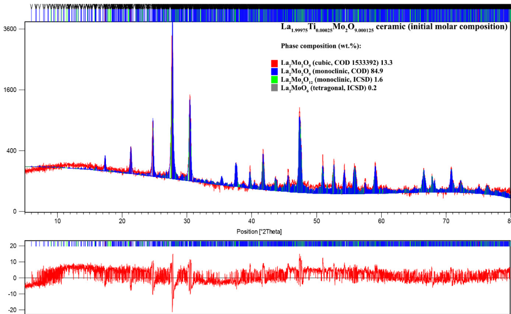
Figure A9. XRD pattern pressed by Rietveld refinement for the La 1.99975 Ti 0.00025 Mo 2 O 9.000125 ceramic composition.
