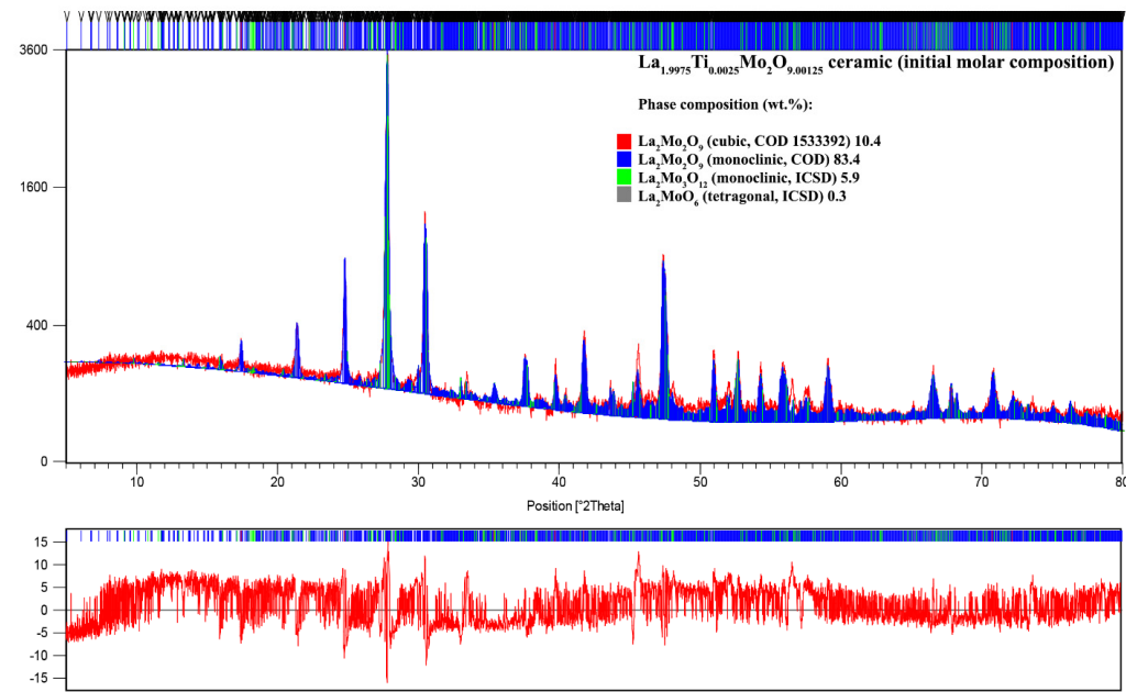
Figure A15. XRD pattern processed by Rietveld refinement for the La 1.9975 Ti 0.0025 Mo 2 O 9.00125 ceramic composition.
