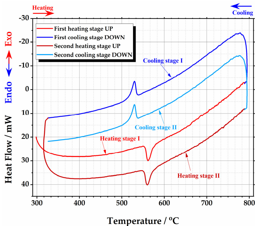
Figure A8. DSC curve of the phase transition cycles for \text{La}_{1.997}\text{Ti}_{0.003}\text{Mo}_2\text{O}_{9.0015} ceramic heat-treated at 1000\text{ }^{\circ}\text{C} .
